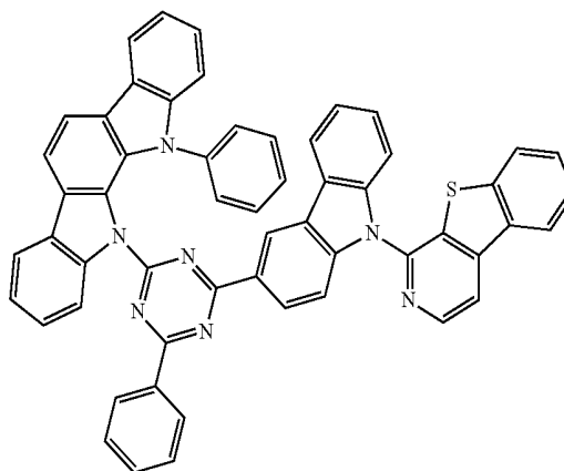
Compound A65
