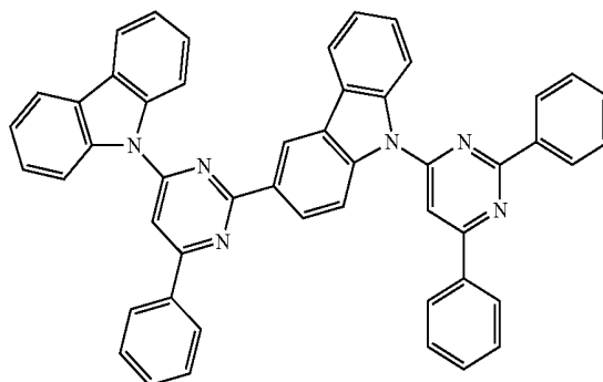
Compound A6
