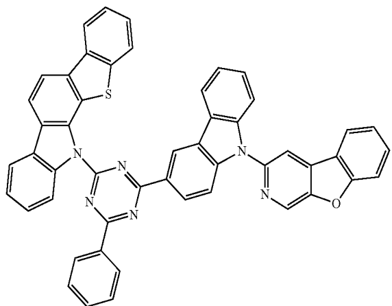
Compound A70
