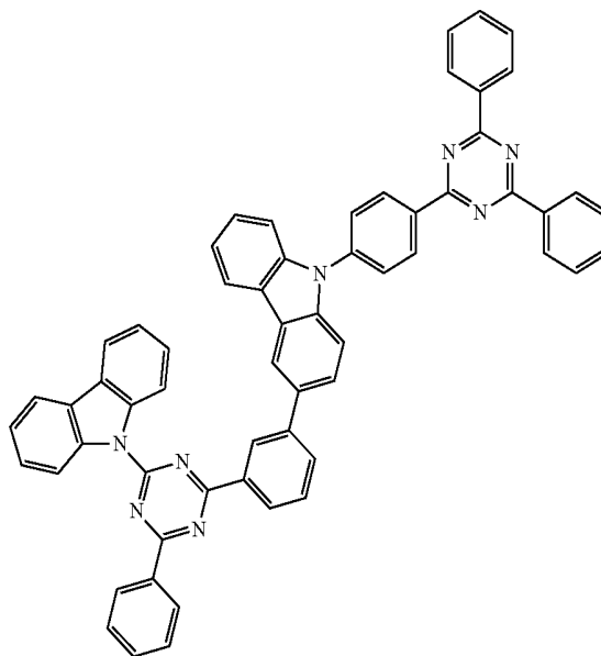
Compound A10
