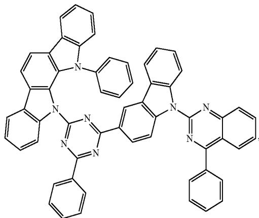
Compound A66
