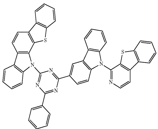
Compound A68
