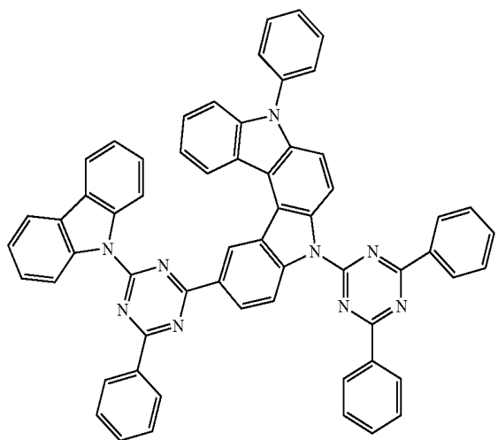
Compound A52
