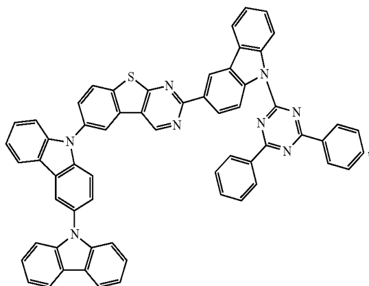
Compound A92
