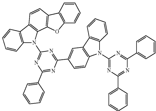
Compound A15
