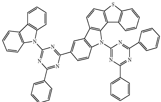
Compound A41
