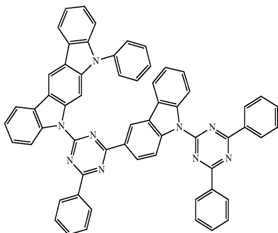
Compound A24
