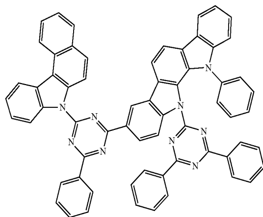
Compound A83
