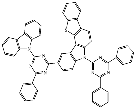
-continued Compound A53
