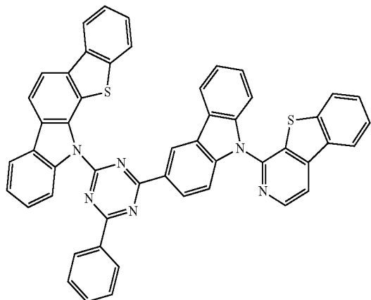
-continued Compound A68
