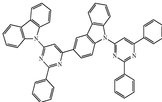
Compound A4
