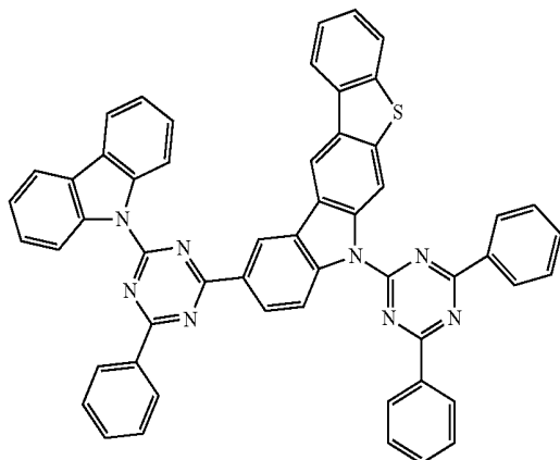
Compound A47
