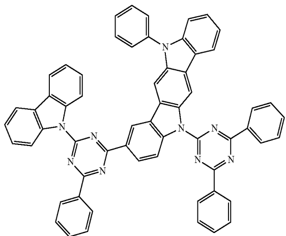
Compound A46
