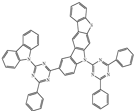
-continued Compound A47
