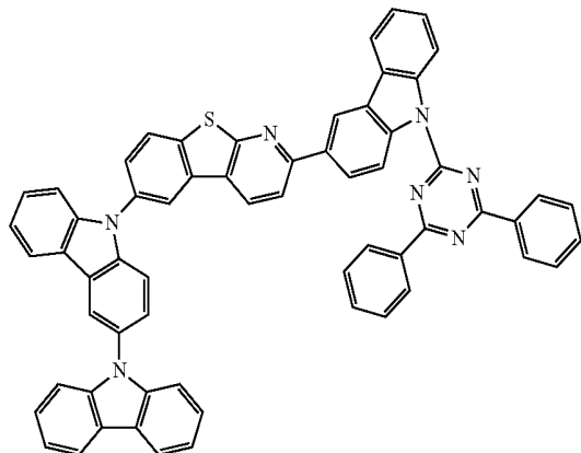
Compound A93
