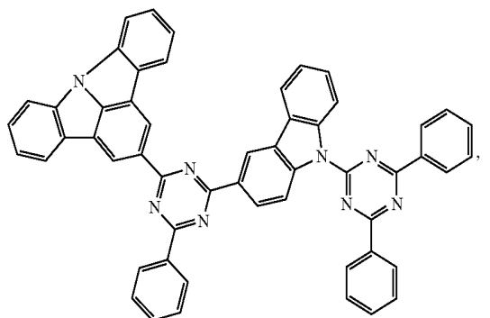
Compounds A34
