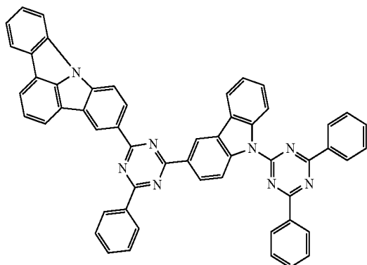
Compound A35
