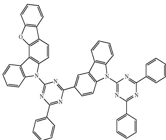
Compound A26
