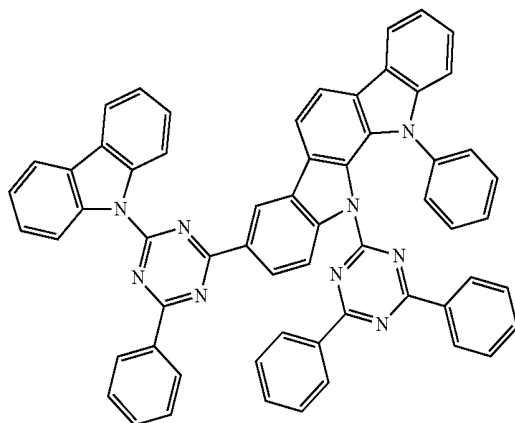
Compound A80
