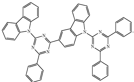
Compound A3
