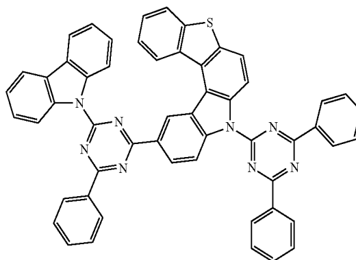
Compound A50
