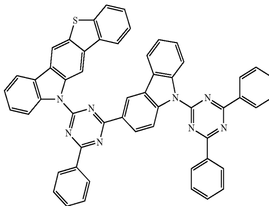
Compound A19
