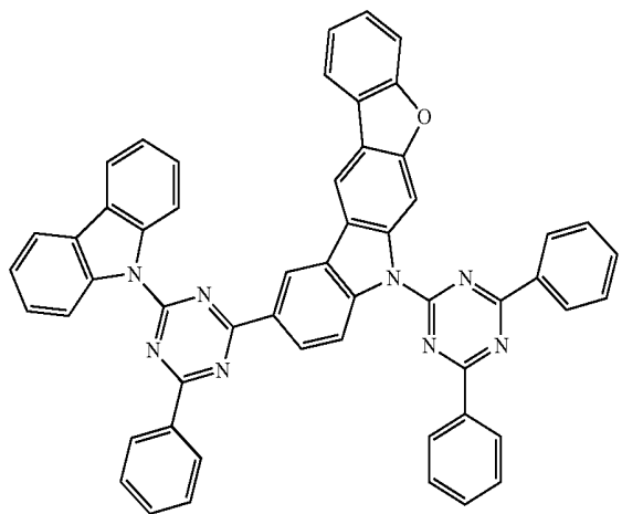
Compound A48
