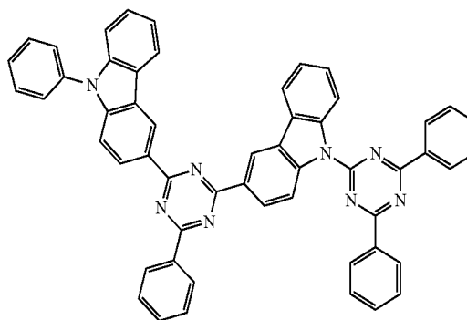
Compound A12
