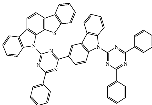
Compound A14
