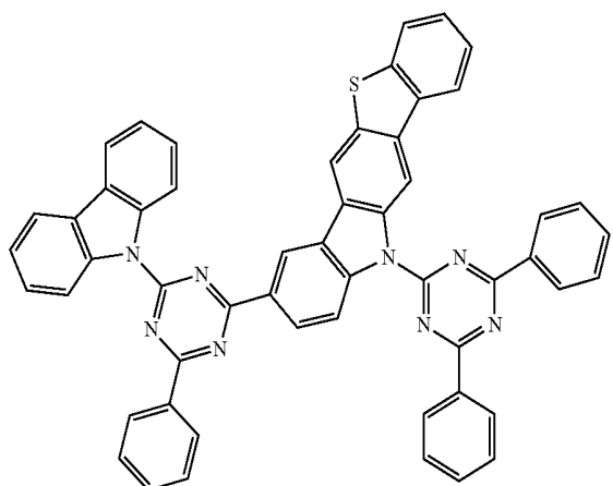
Compound A44
