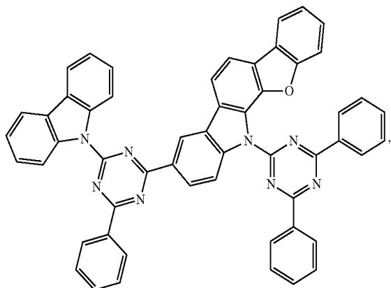
Compound A39
