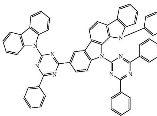
Compound A40
