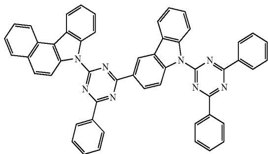
Compound A32
