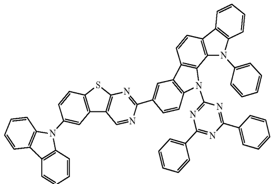
Compound A87
