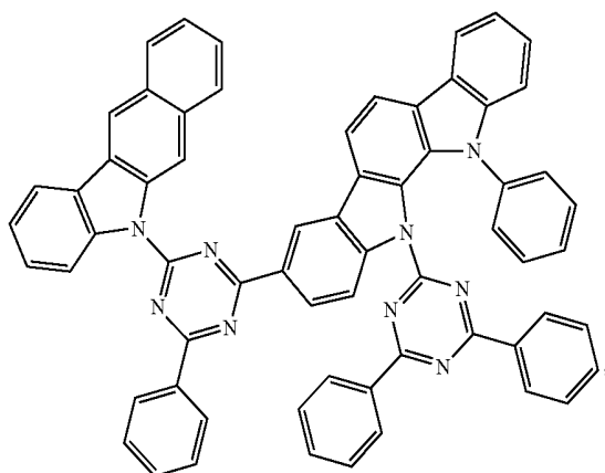
Compound A82
