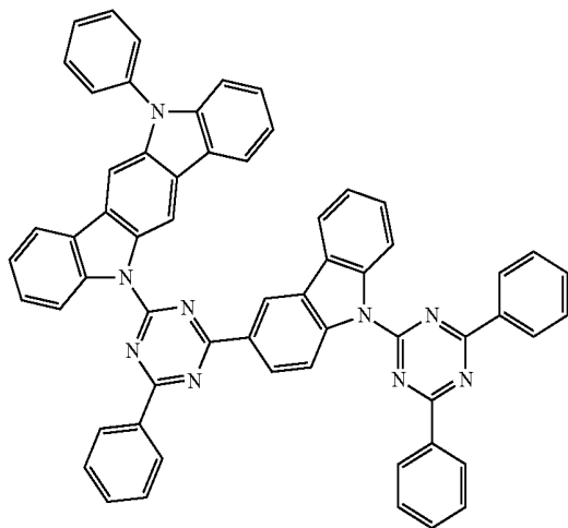
Compound A23
