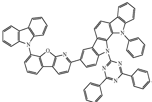
Compound A86
