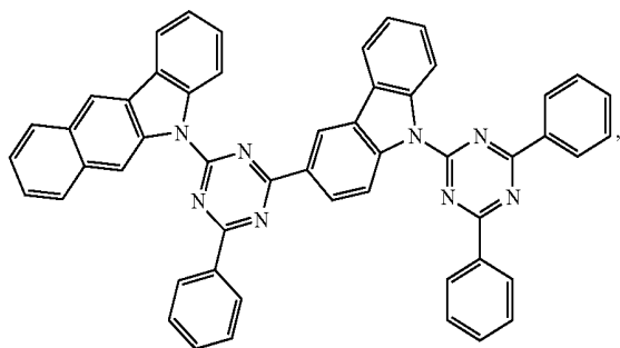
Compound A31
