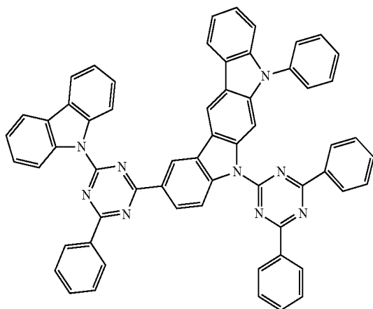
Compound A49
