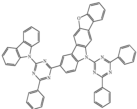
Compound A45
