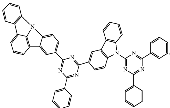
Compound A33
