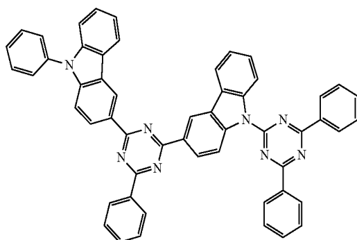
Compound A12
