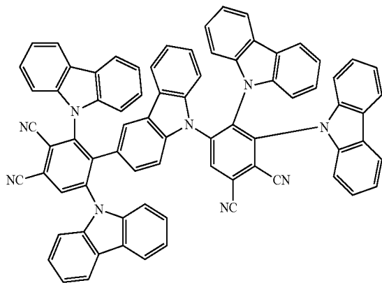
Compound B37
