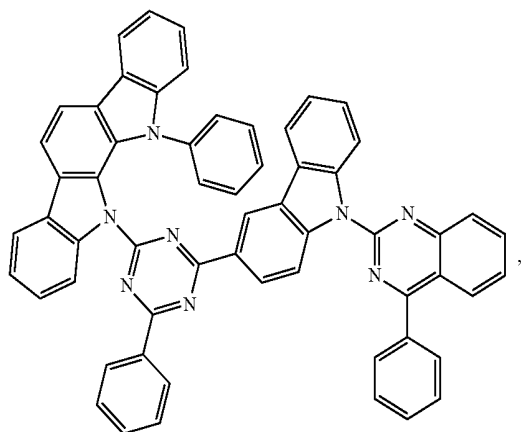
Compound A66
