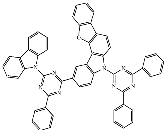
Compound A54
