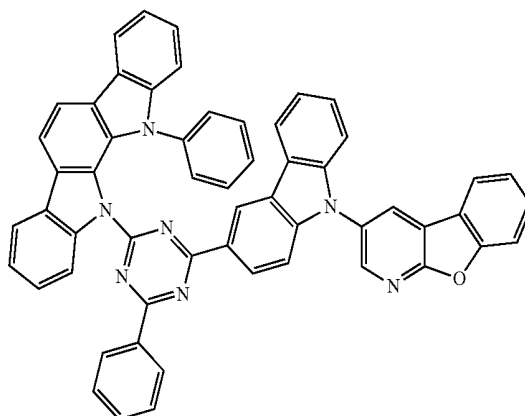
Compound A67
