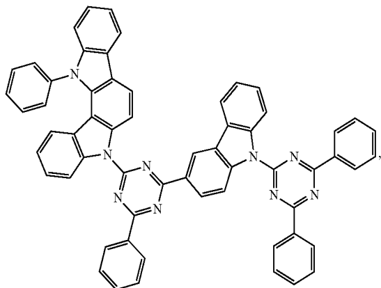
Compound A29
