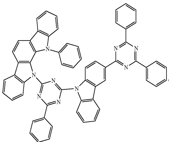
Compound A64
