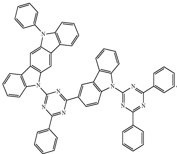
Compound A21
