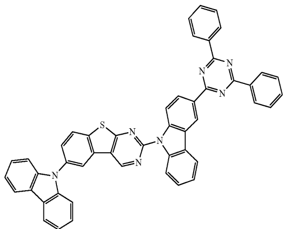
Compound A78
