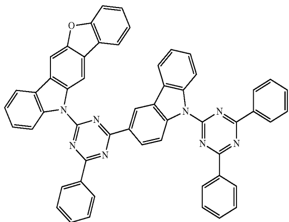
Compound A20
