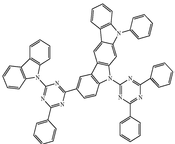
Compound A49
