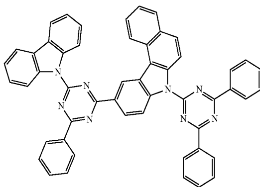
Compound A39
