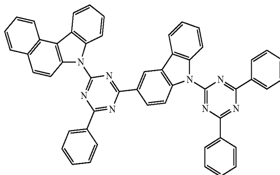
Compound A30
