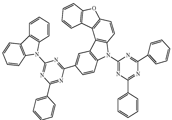
Compound A51
