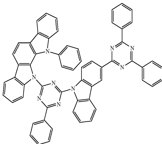
Compound A64
